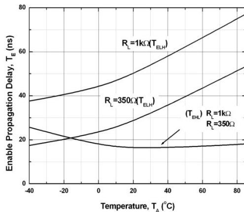
Figure 11. Enable Propagation Delay vs. Temperature
