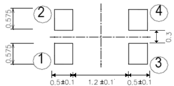
soldering pattern
