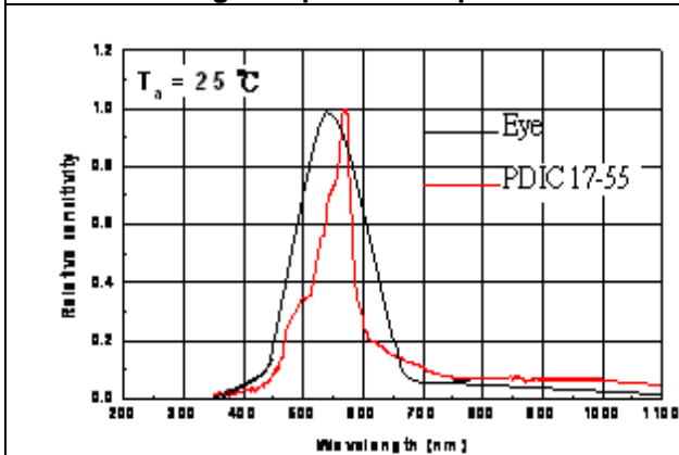
Fig.9 Spectral Response
