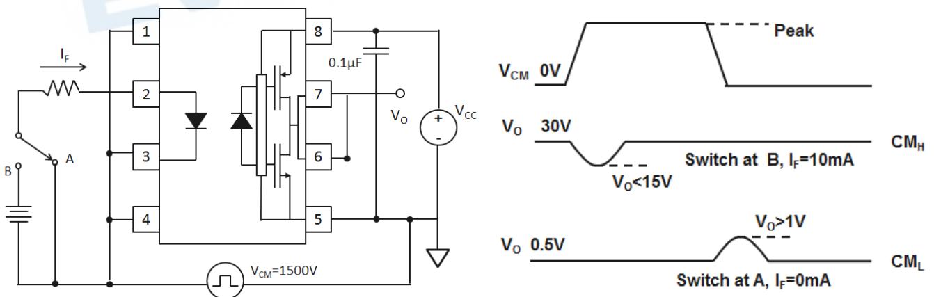
Fig. 22 CMR Test circuit
