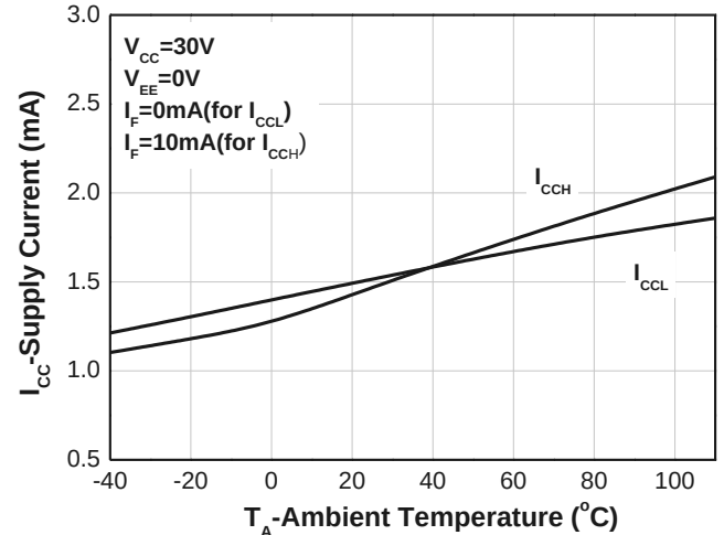
Fig.6 Supply Current vs. Ambient Temperature
