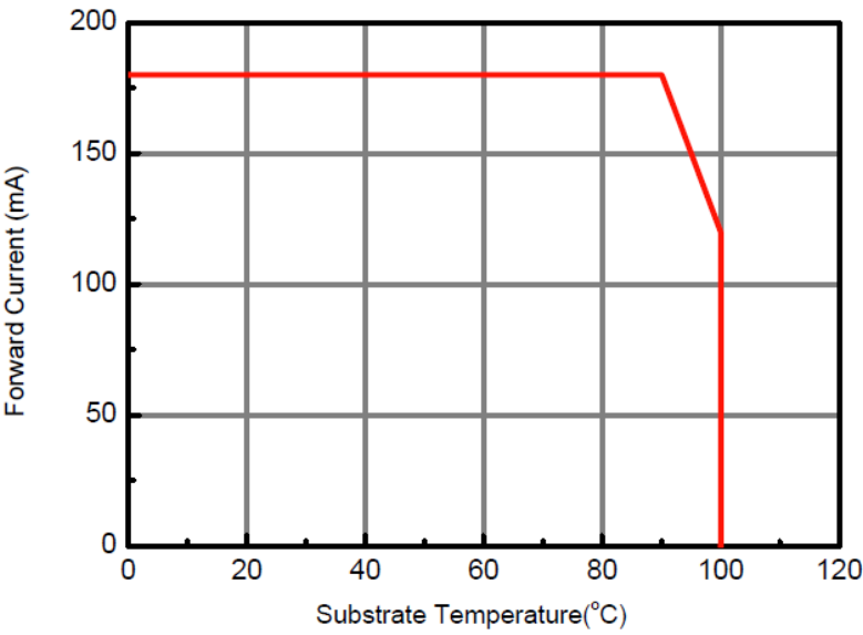
Forward Current Derating Curve @ Junction Temperature <120°C
